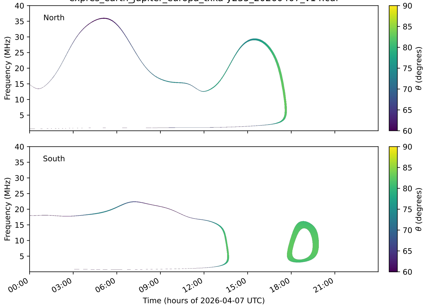
expres_earth_jupiter_europa_txka-y235_20260407_v14.cdf
