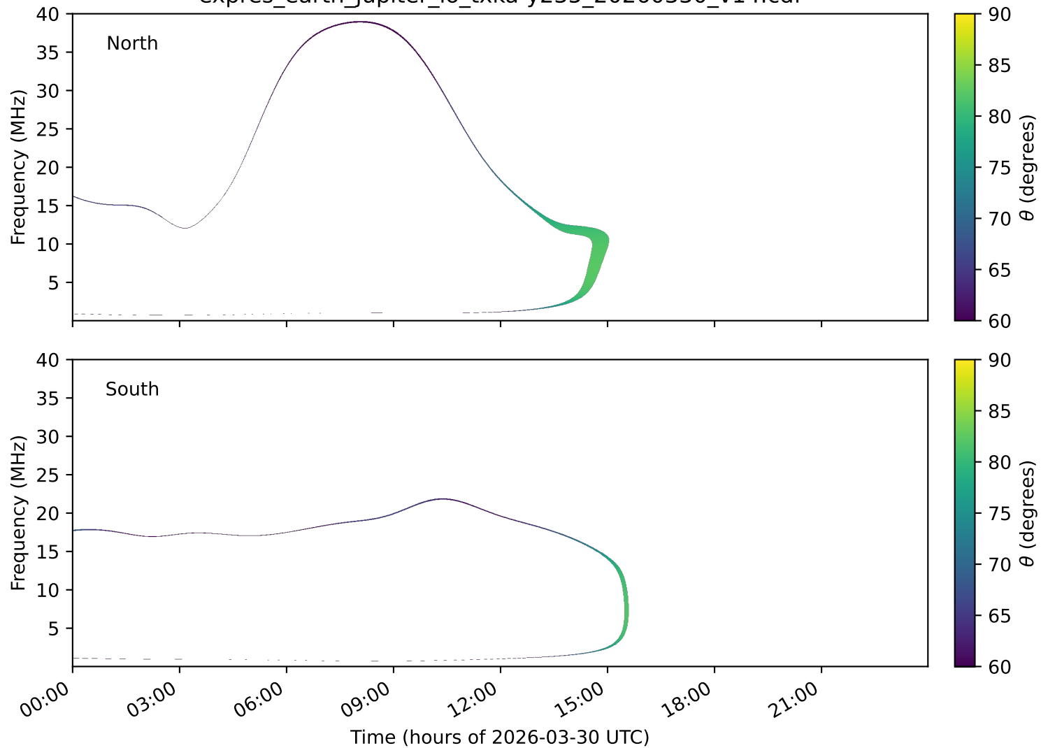
expres_earth_jupiter_io_txka-y235_20260330_v14.cdf
