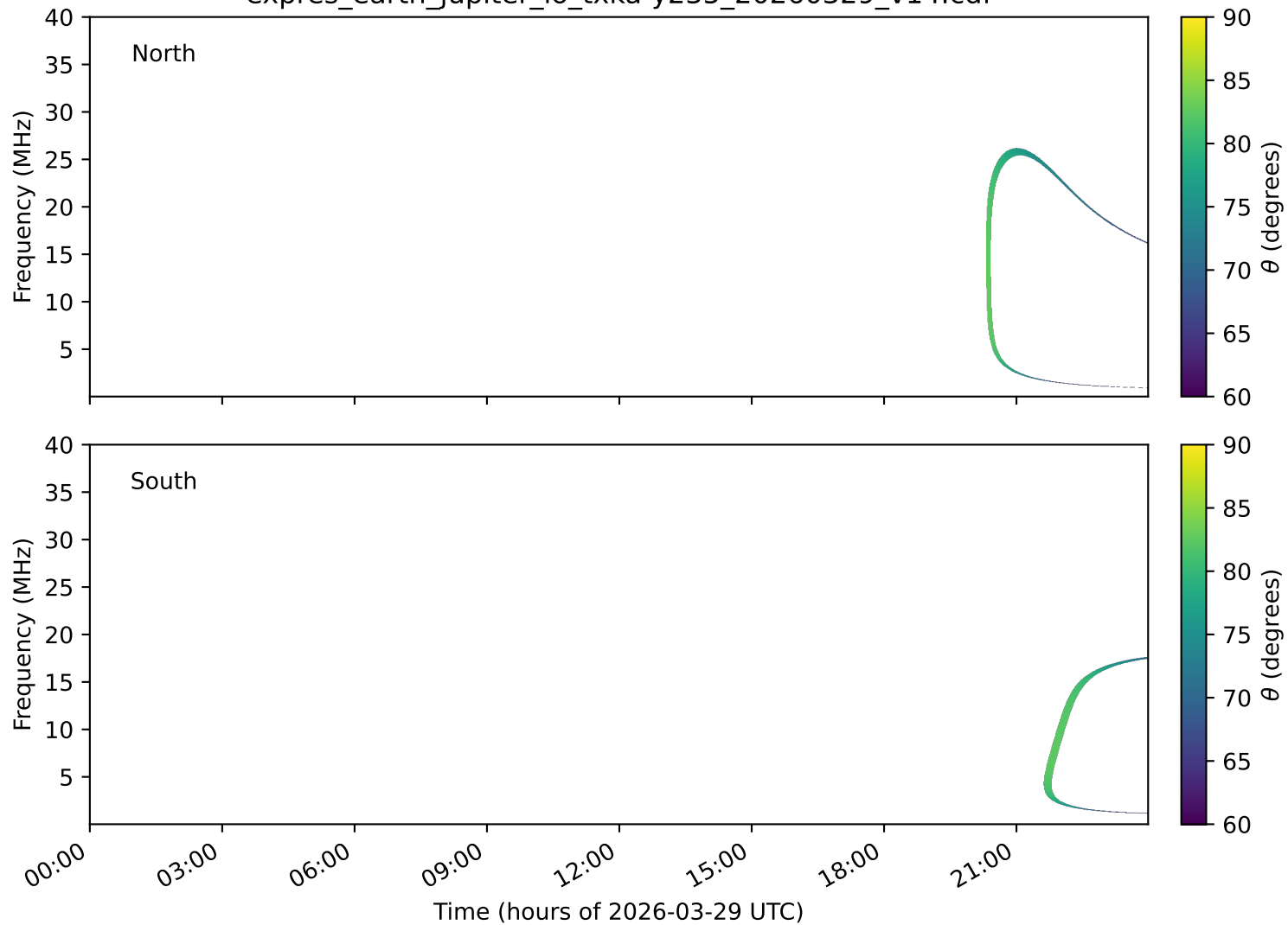
expres_earth_jupiter_io_txka-y235_20260329_v14.cdf
