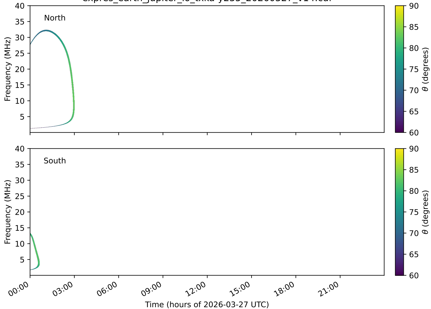
expres_earth_jupiter_io_txka-y235_20260327_v14.cdf
