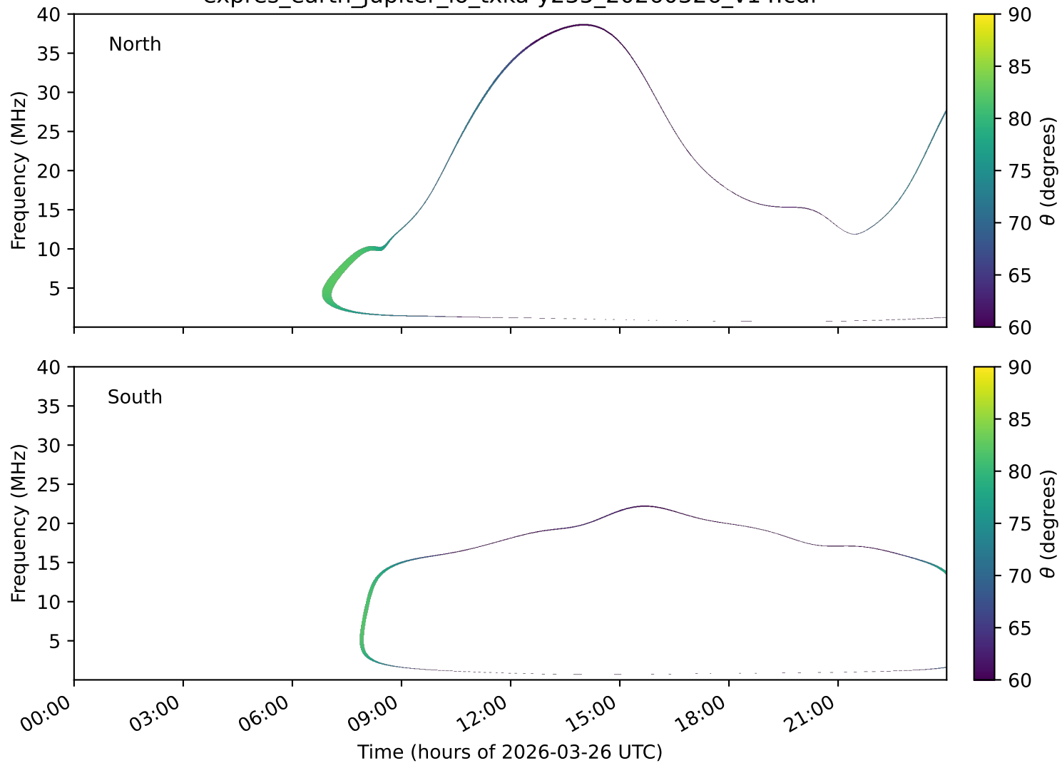
expres_earth_jupiter_io_txka-y235_20260326_v14.cdf
