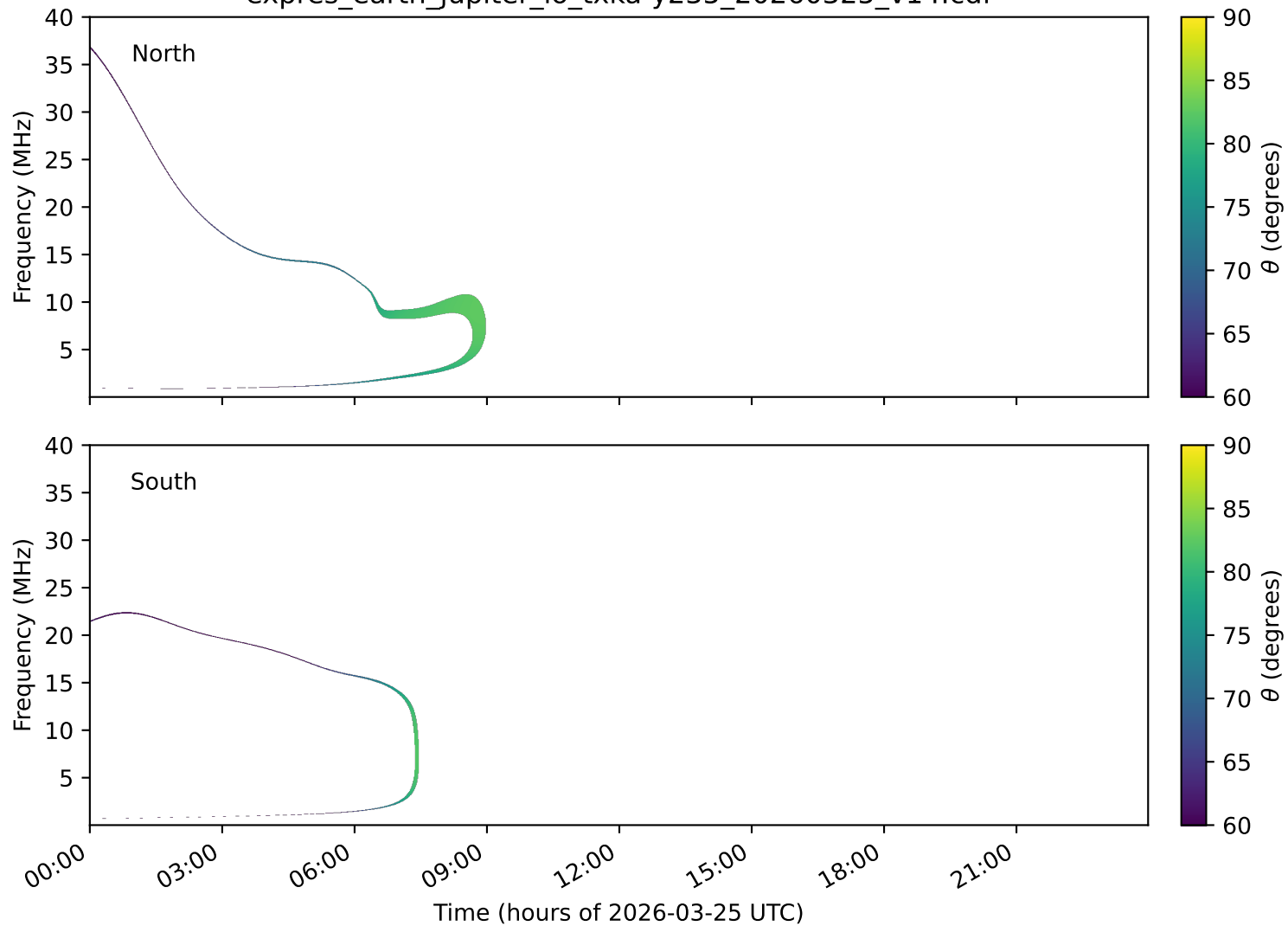
expres_earth_jupiter_io_txka-y235_20260325_v14.cdf
