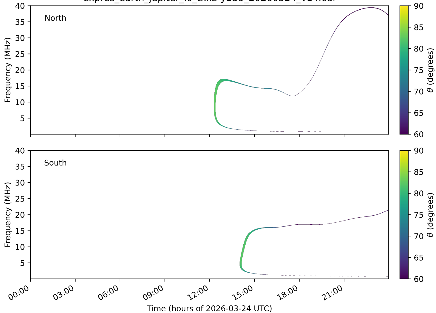
expres_earth_jupiter_io_txka-y235_20260324_v14.cdf
