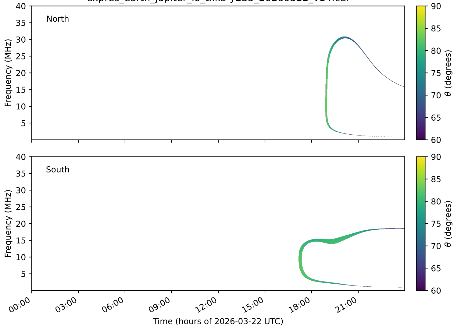
expres_earth_jupiter_io_txka-y235_20260322_v14.cdf
