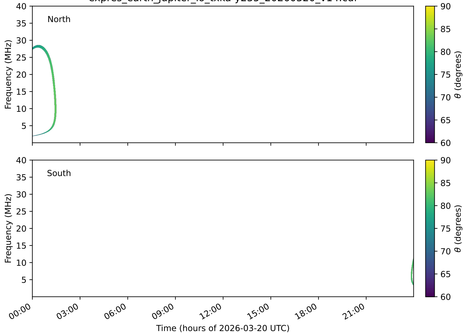
expres_earth_jupiter_io_txka-y235_20260320_v14.cdf
