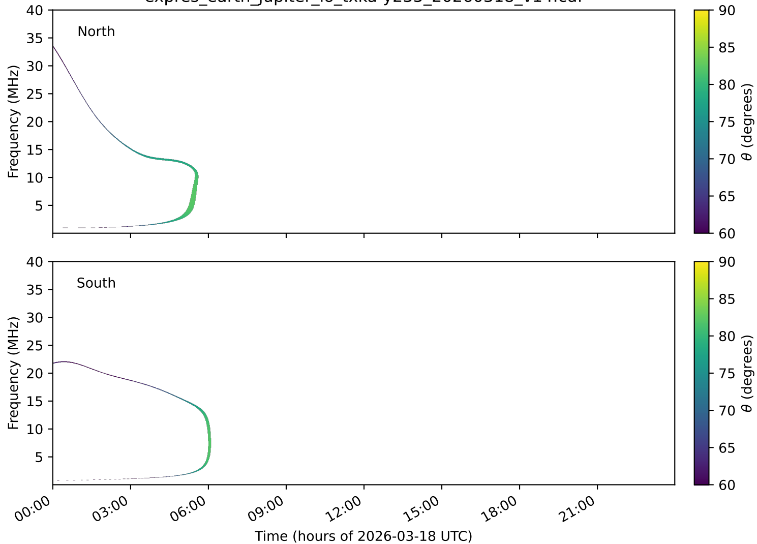
expres_earth_jupiter_io_txka-y235_20260318_v14.cdf
