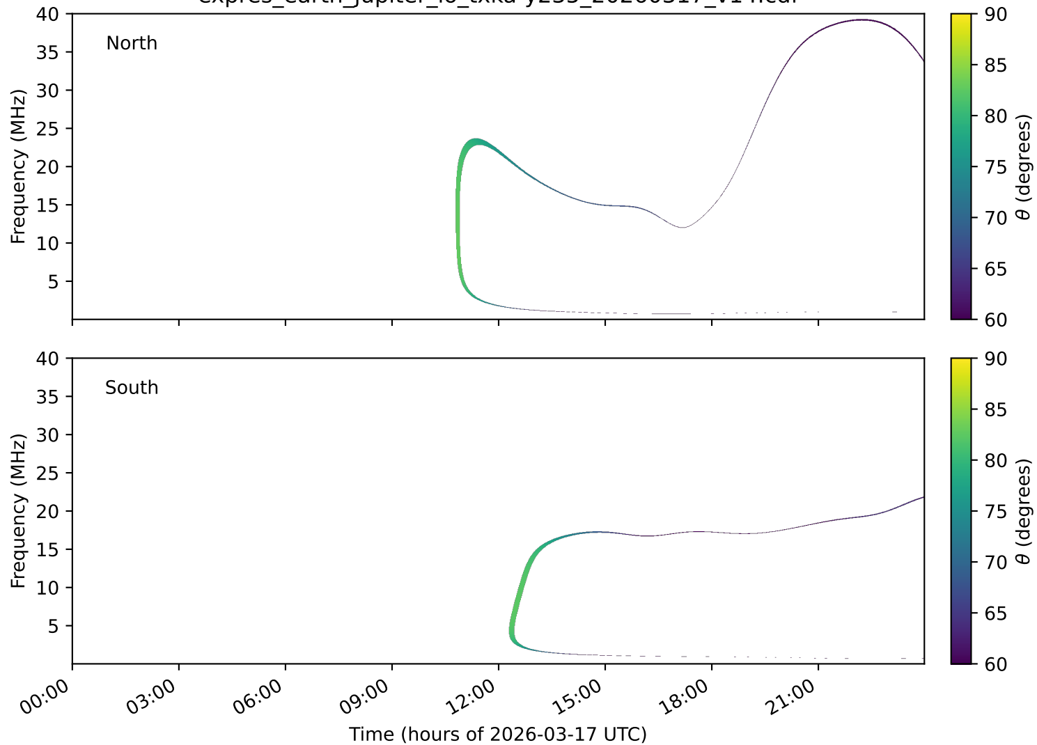
expres_earth_jupiter_io_txka-y235_20260317_v14.cdf
