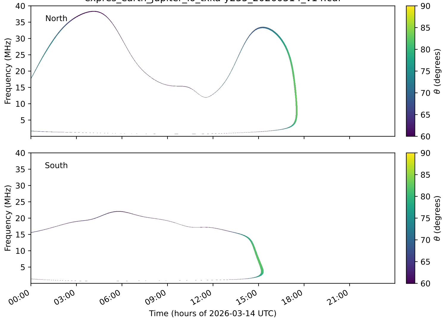
expres_earth_jupiter_io_txka-y235_20260314_v14.cdf
