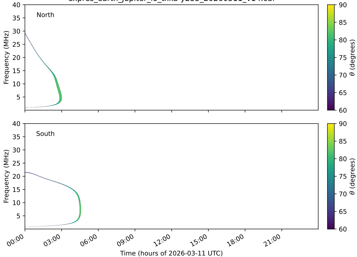
expres_earth_jupiter_io_txka-y235_20260311_v14.cdf
