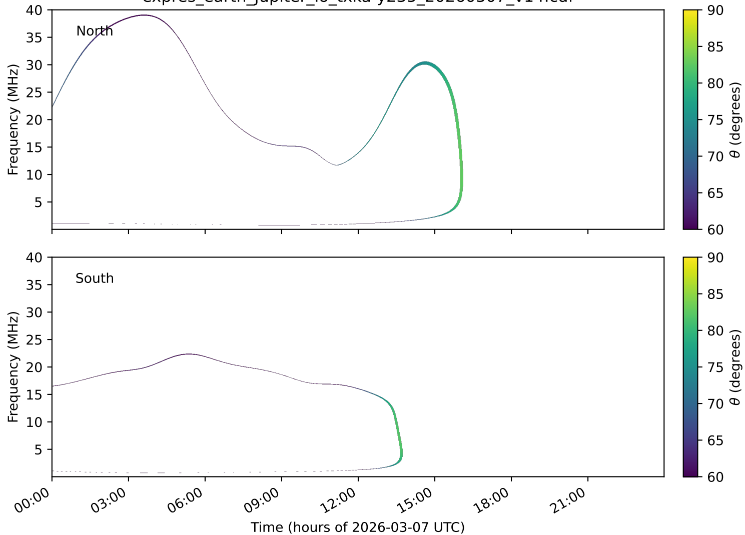
expres_earth_jupiter_io_txka-y235_20260307_v14.cdf
