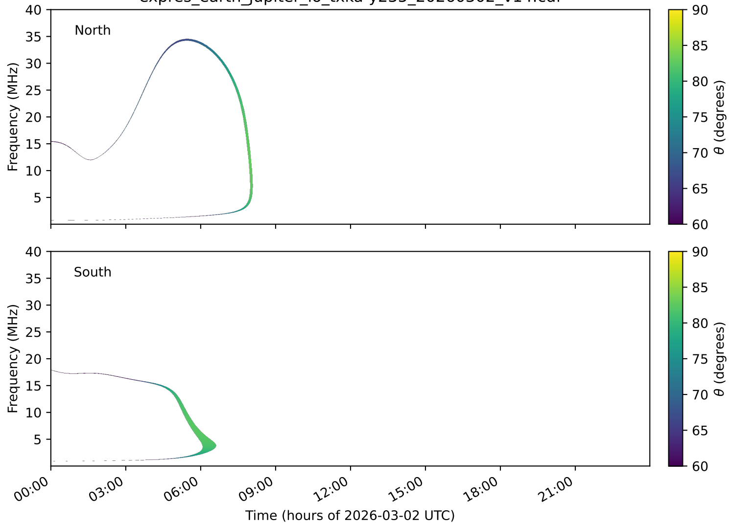
expres_earth_jupiter_io_txka-y235_20260302_v14.cdf
