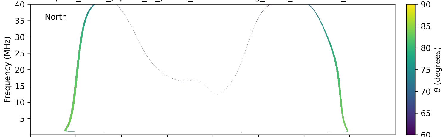
expres_earth_jupiter_io_jrm33_lossc-wid1deg_3kev_20260328_v11.cdf
