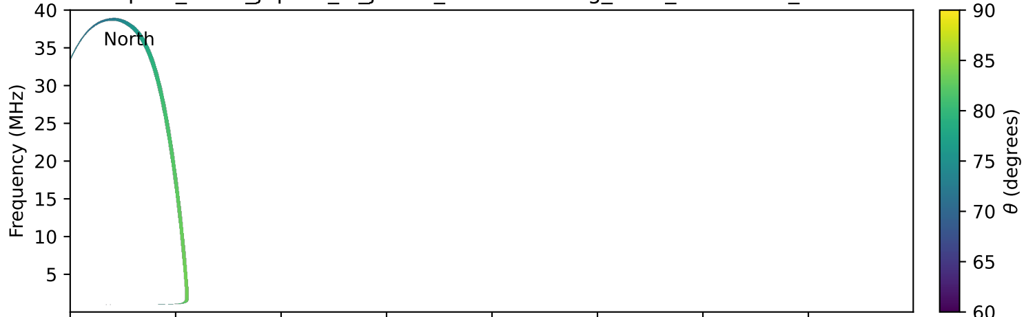
expres_earth_jupiter_io_jrm33_lossc-wid1deg_3kev_20260327_v11.cdf
