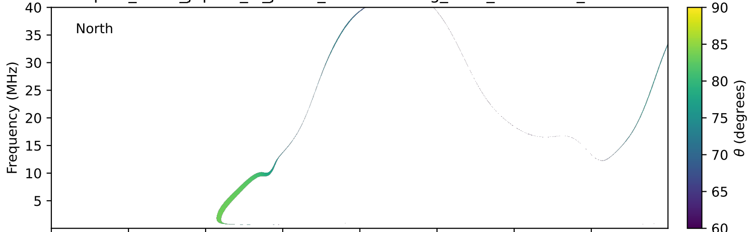
expres_earth_jupiter_io_jrm33_lossc-wid1deg_3kev_20260326_v11.cdf
