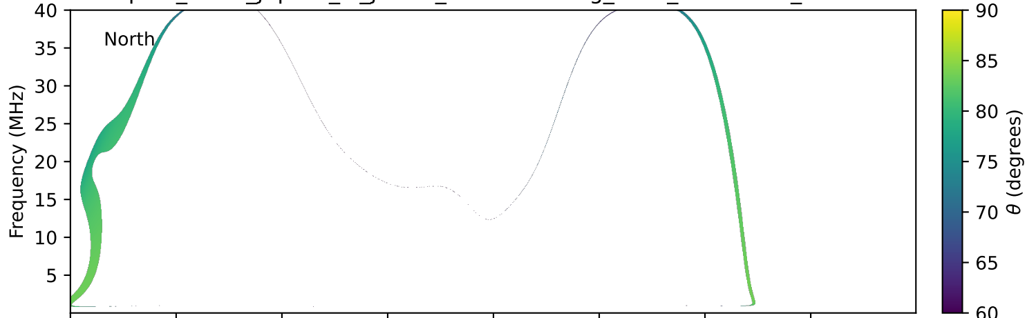
expres_earth_jupiter_io_jrm33_lossc-wid1deg_3kev_20260321_v11.cdf
