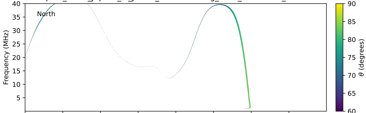
expres_earth_jupiter_io_jrm33_lossc-wid1deg_3kev_20260314_v11.cdf
