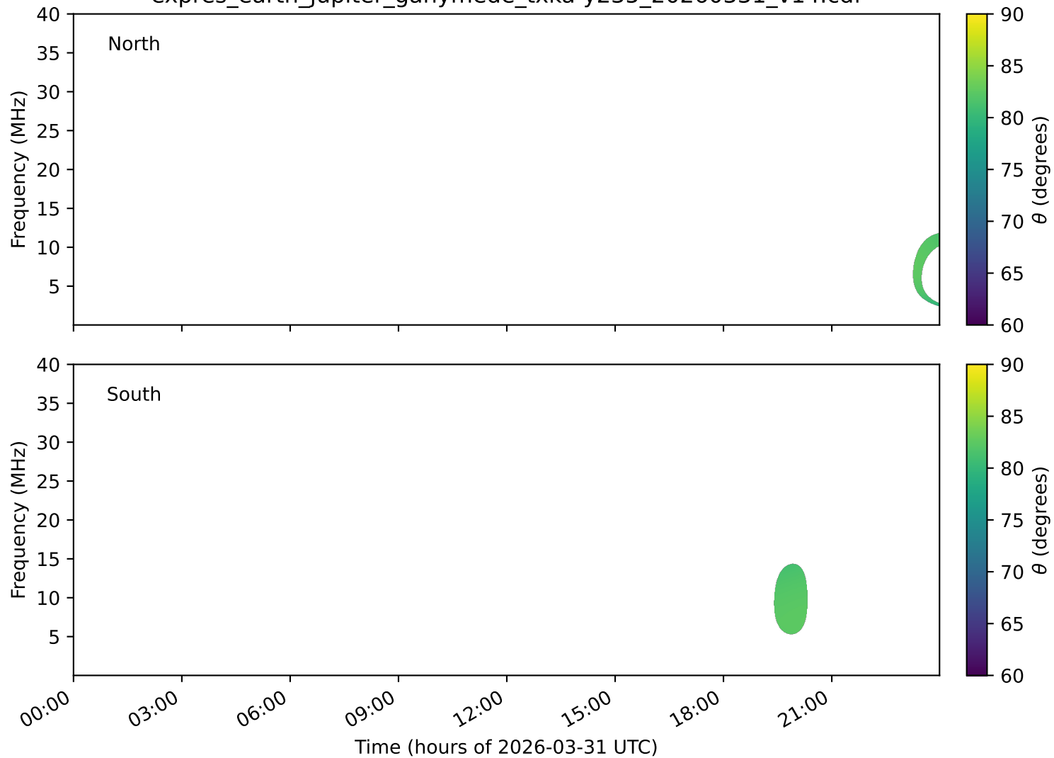
expres_earth_jupiter_ganymede_txka-y235_20260331_v14.cdf
