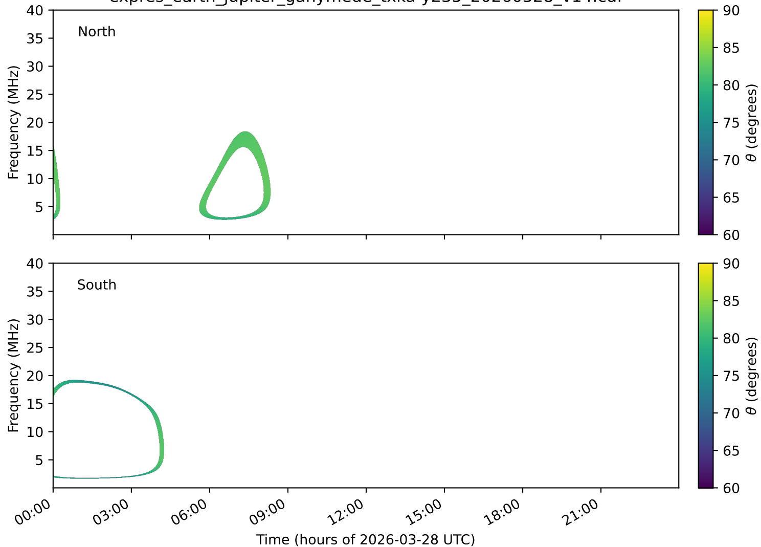
expres_earth_jupiter_ganymede_txka-y235_20260328_v14.cdf
