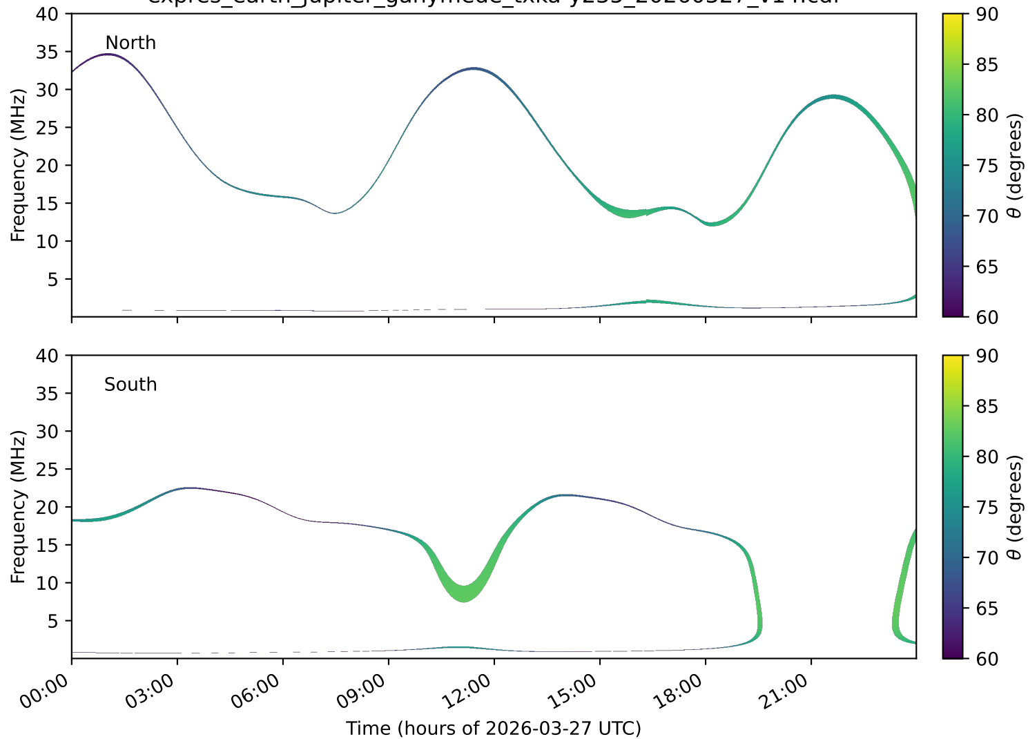
expres_earth_jupiter_ganymede_txka-y235_20260327_v14.cdf
