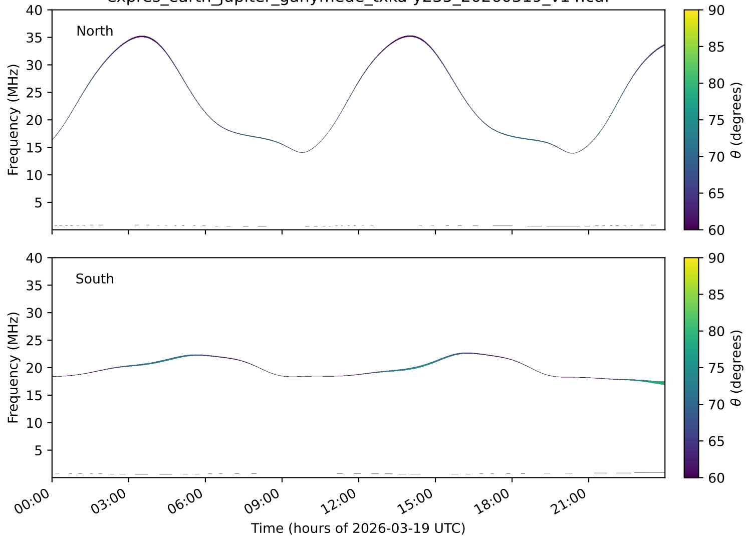
expres_earth_jupiter_ganymede_txka-y235_20260319_v14.cdf
