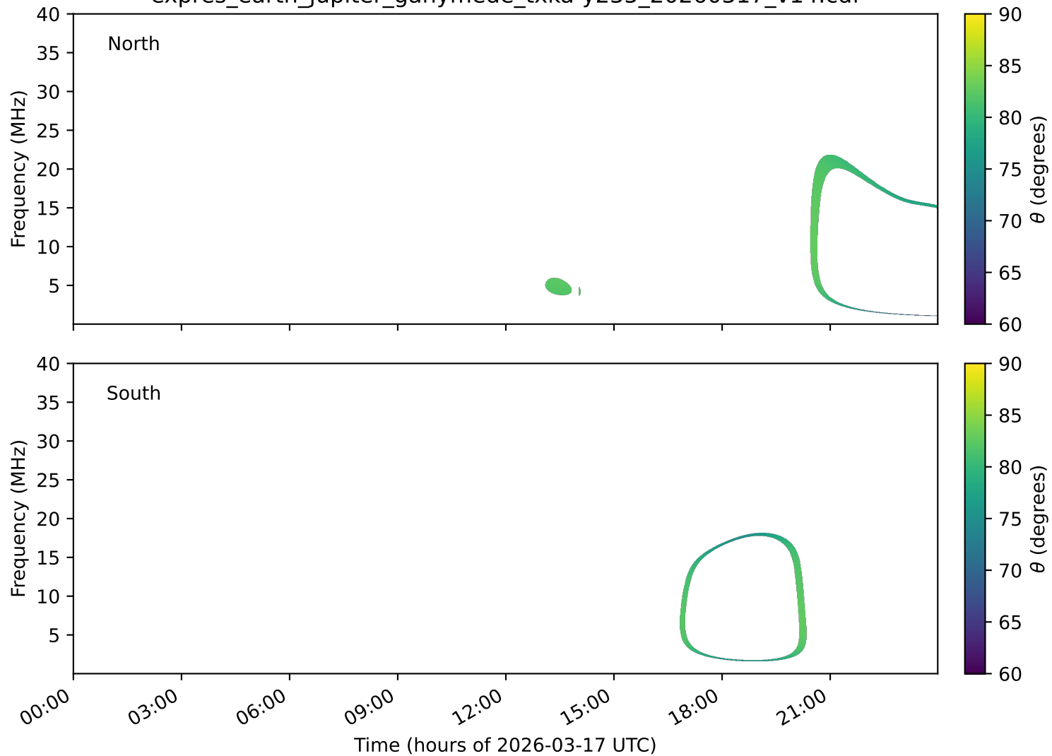
expres_earth_jupiter_ganymede_txka-y235_20260317_v14.cdf
