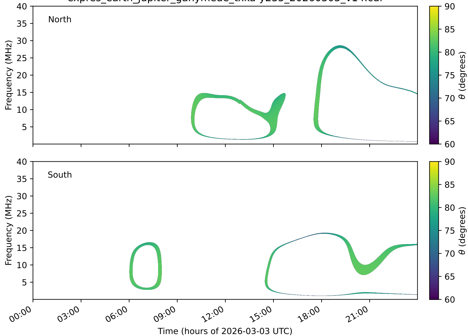
expres_earth_jupiter_ganymede_txka-y235_20260303_v14.cdf
