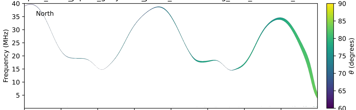
expres_earth_jupiter_ganymede_jrm33_lossc-wid1deg_3kev_20260320_v11.cdf
