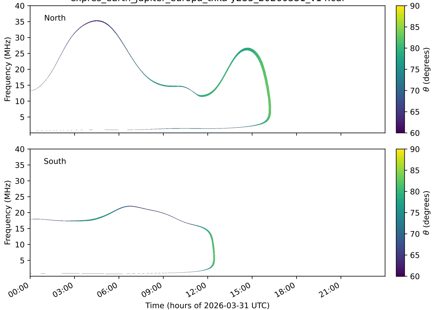
expres_earth_jupiter_europa_txka-y235_20260331_v14.cdf
