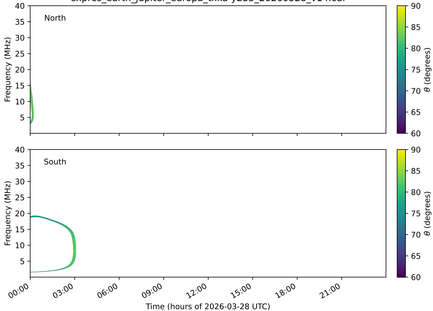
expres_earth_jupiter_europa_txka-y235_20260328_v14.cdf
