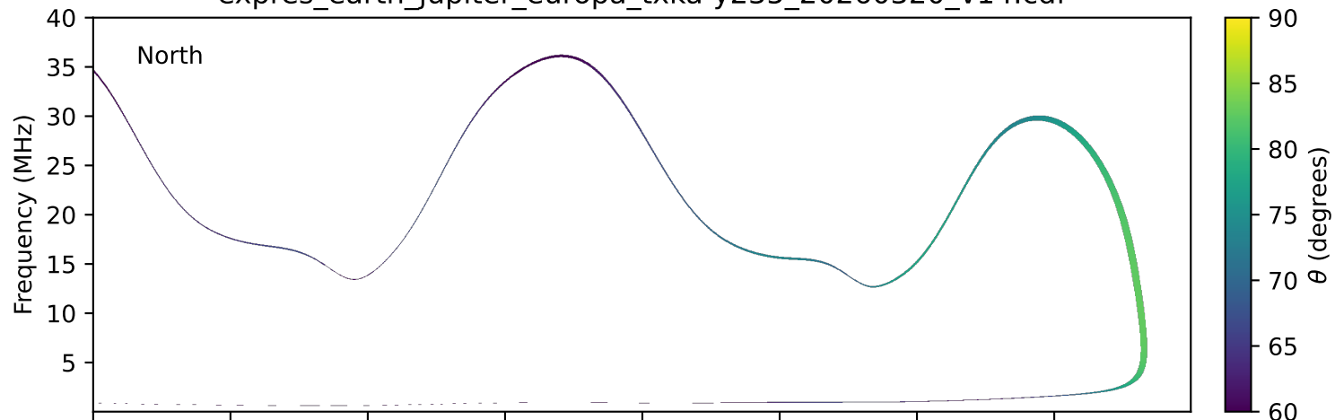
expres_earth_jupiter_europa_txka-y235_20260320_v14.cdf
