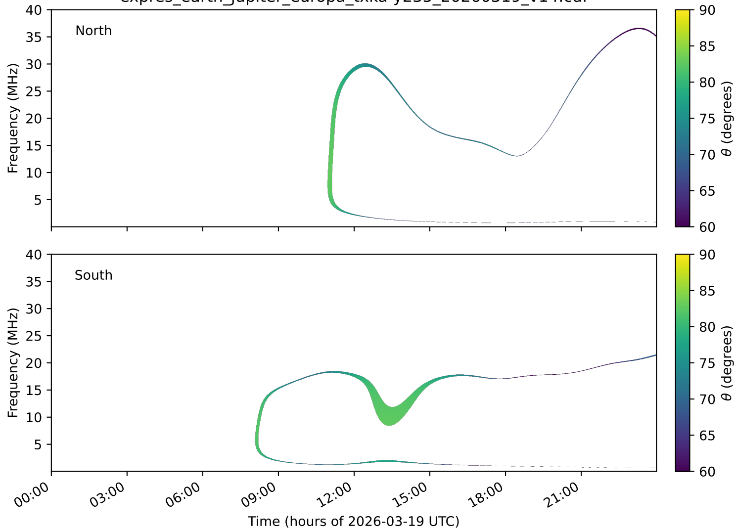
expres_earth_jupiter_europa_txka-y235_20260319_v14.cdf
