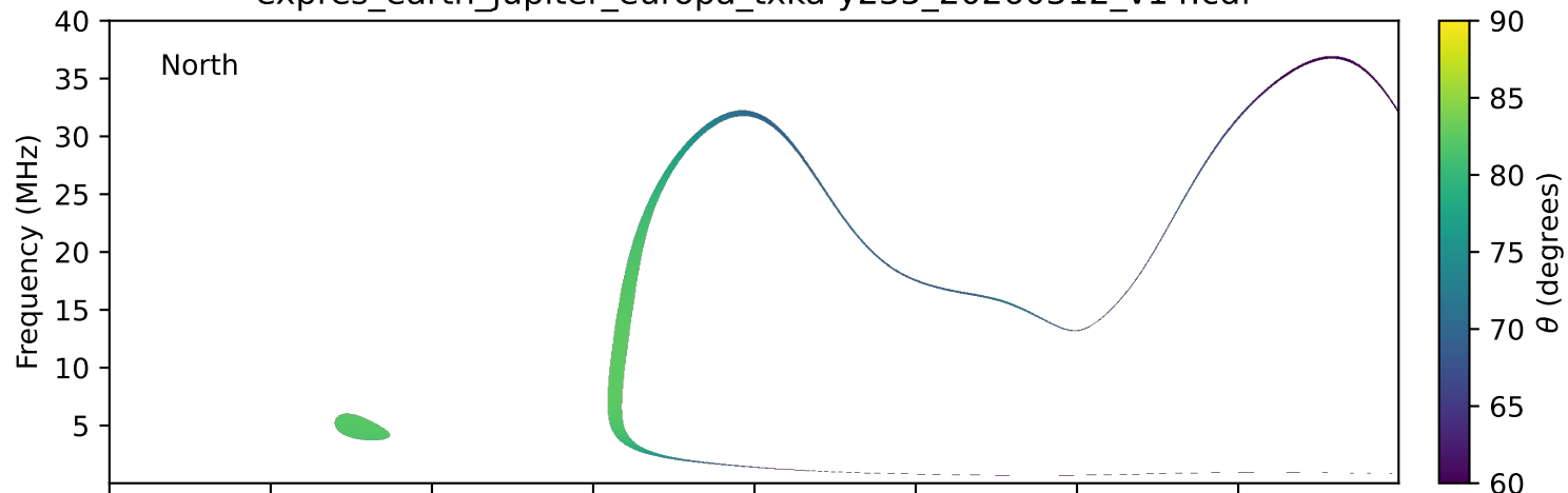
expres_earth_jupiter_europa_txka-y235_20260312_v14.cdf
