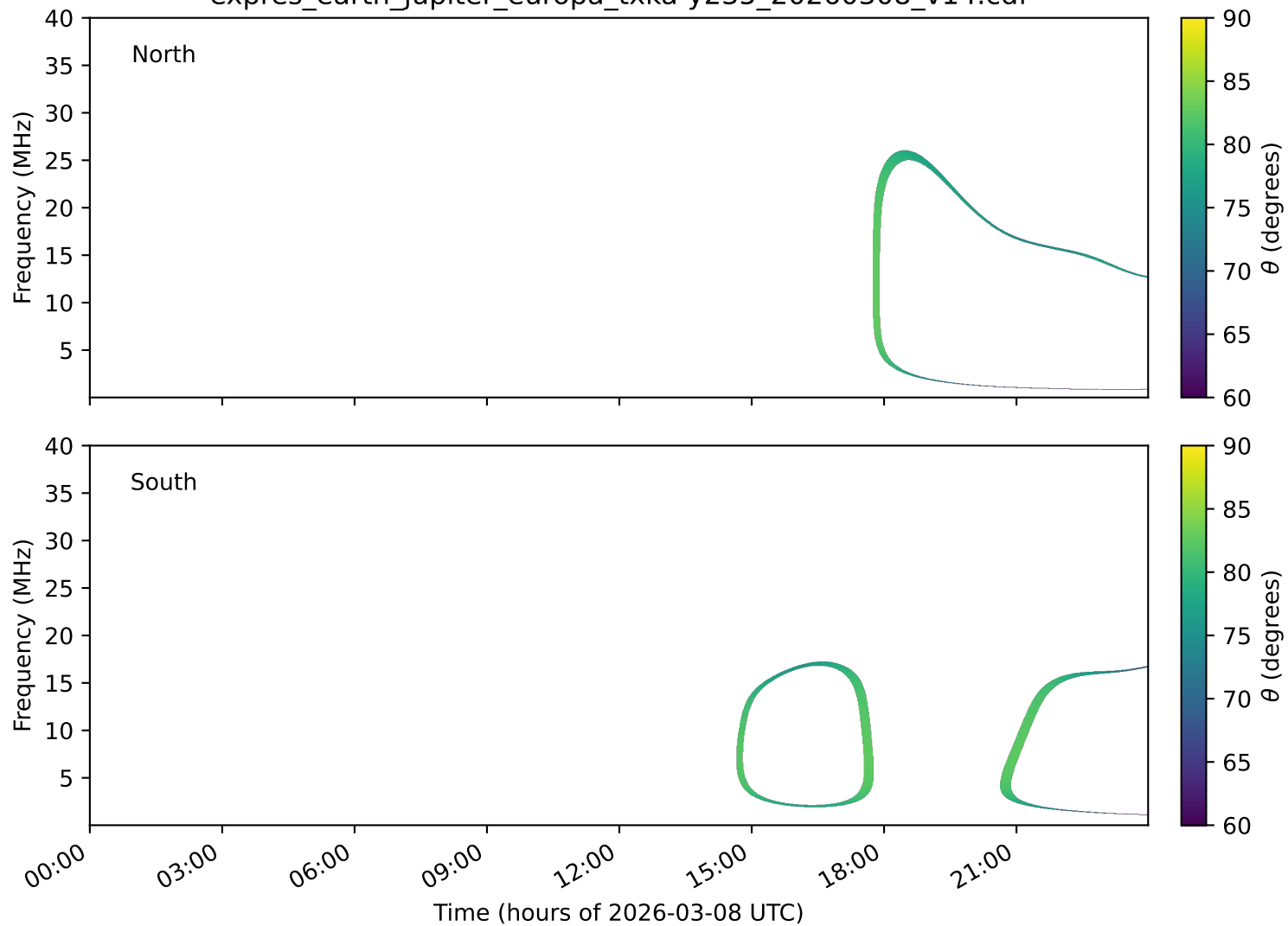
expres_earth_jupiter_europa_txka-y235_20260308_v14.cdf
