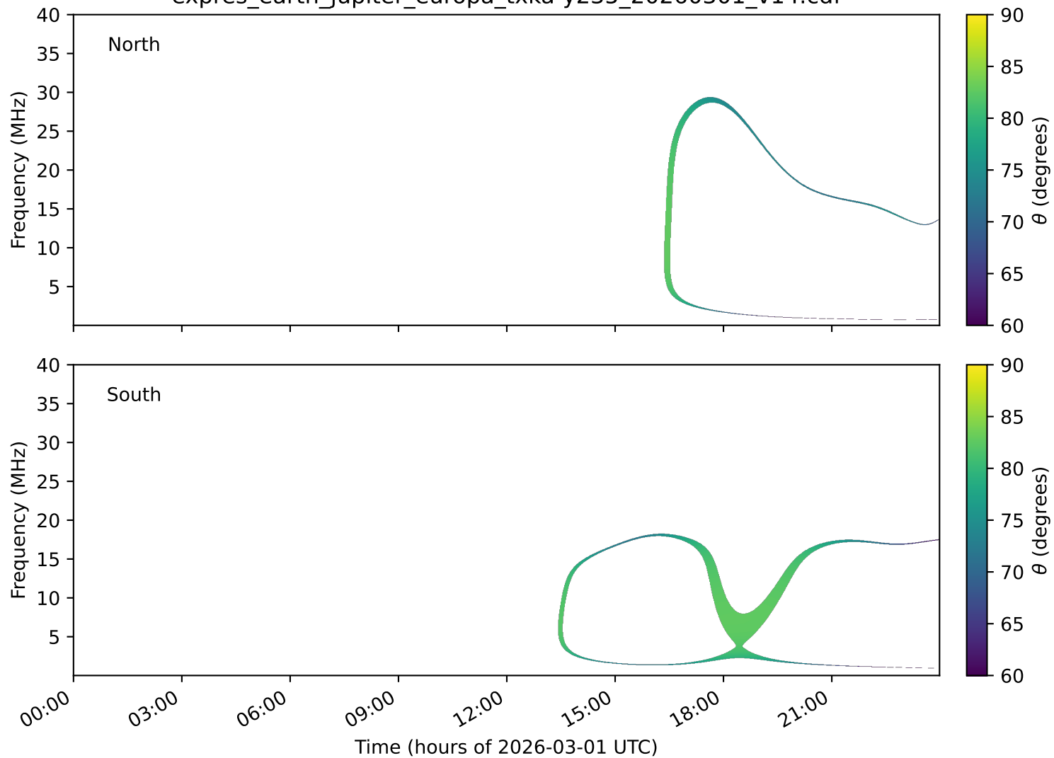
expres_earth_jupiter_europa_txka-y235_20260301_v14.cdf
