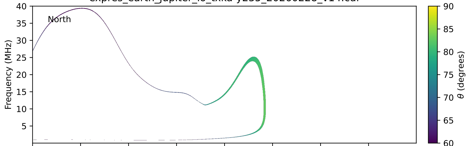
expres_earth_jupiter_io_txka-y235_20260228_v14.cdf
