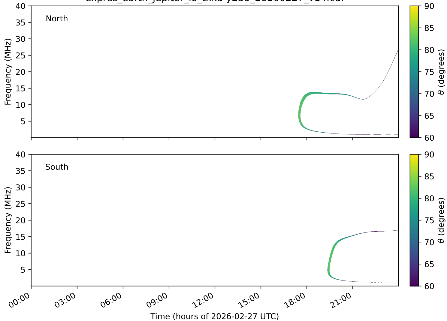
expres_earth_jupiter_io_txka-y235_20260227_v14.cdf
