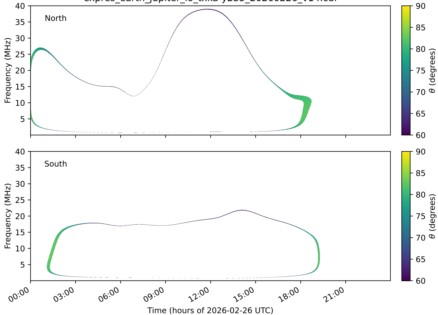
expres_earth_jupiter_io_txka-y235_20260226_v14.cdf
