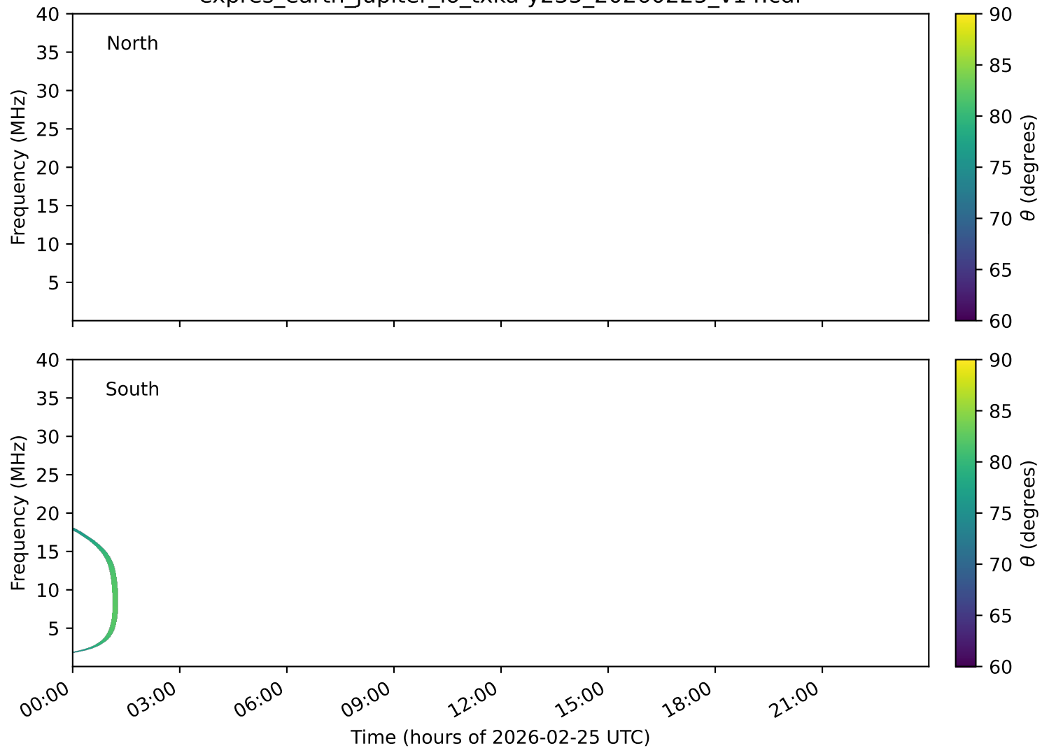
expres_earth_jupiter_io_txka-y235_20260225_v14.cdf
