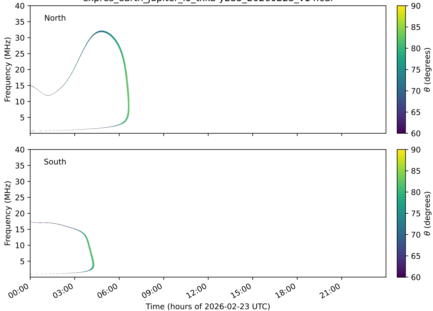
expres_earth_jupiter_io_txka-y235_20260223_v14.cdf
