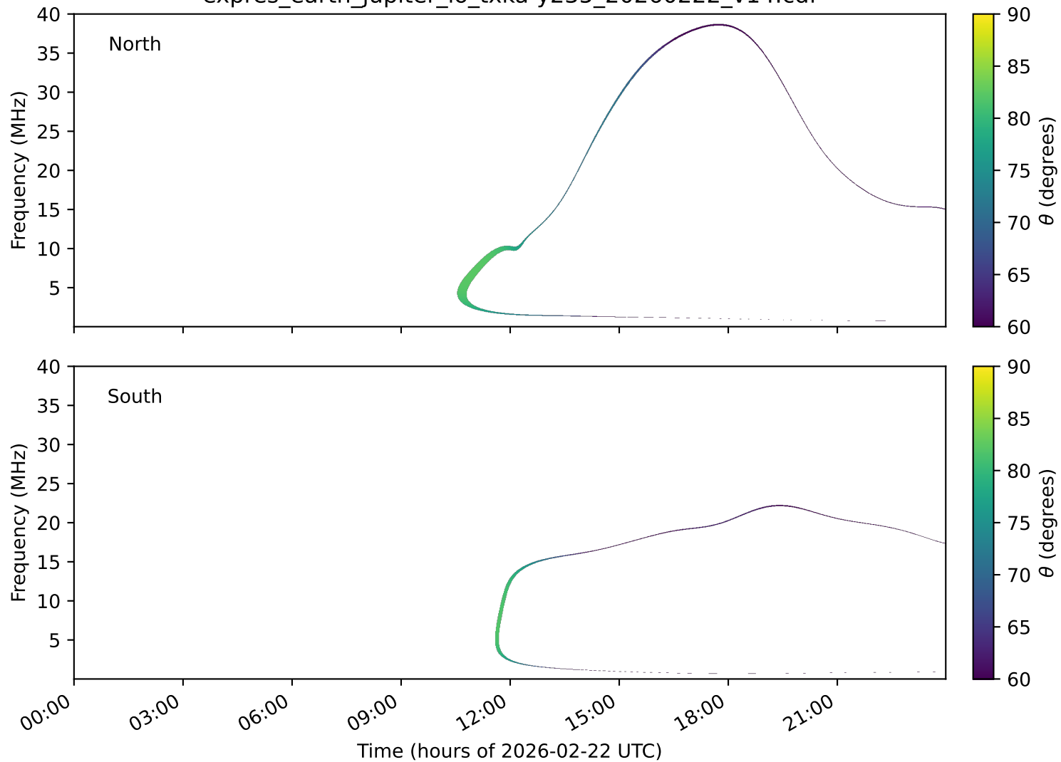
expres_earth_jupiter_io_txka-y235_20260222_v14.cdf
