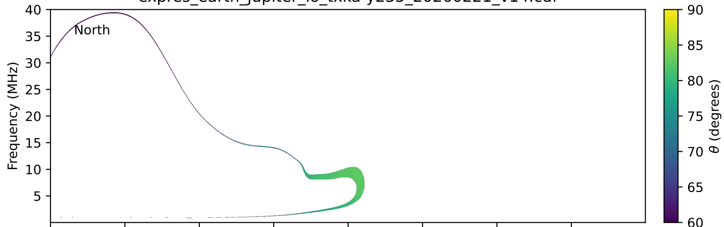
expres_earth_jupiter_io_txka-y235_20260221_v14.cdf
