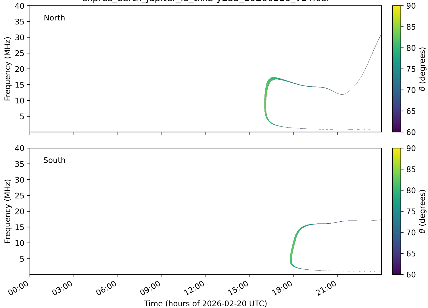
expres_earth_jupiter_io_txka-y235_20260220_v14.cdf
