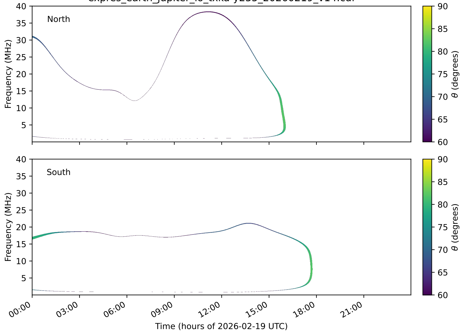
expres_earth_jupiter_io_txka-y235_20260219_v14.cdf
