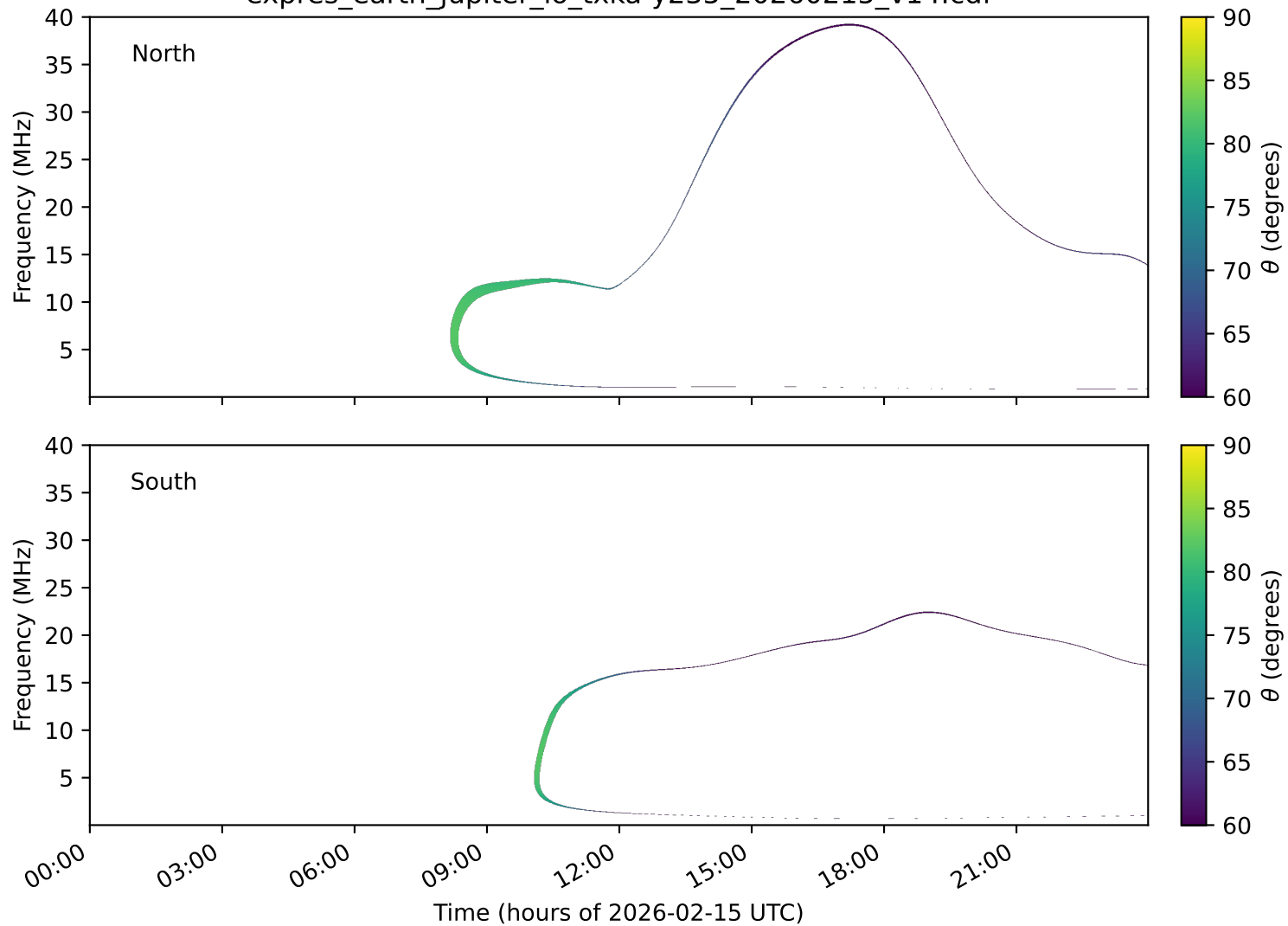
expres_earth_jupiter_io_txka-y235_20260215_v14.cdf
