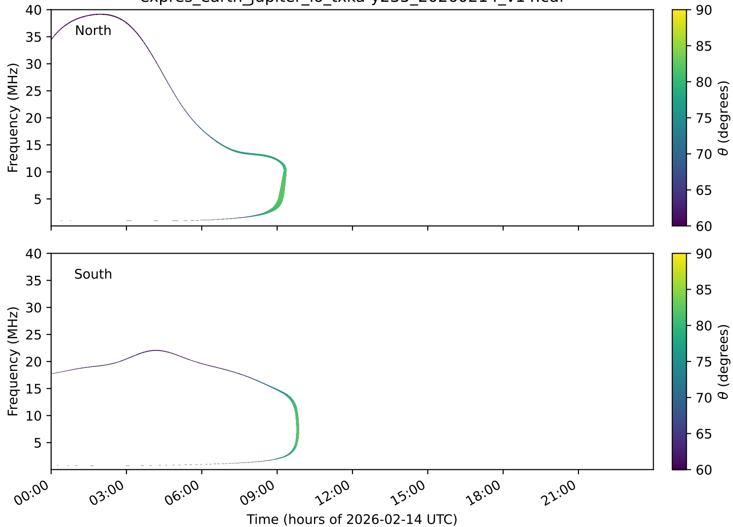
expres_earth_jupiter_io_txka-y235_20260214_v14.cdf
