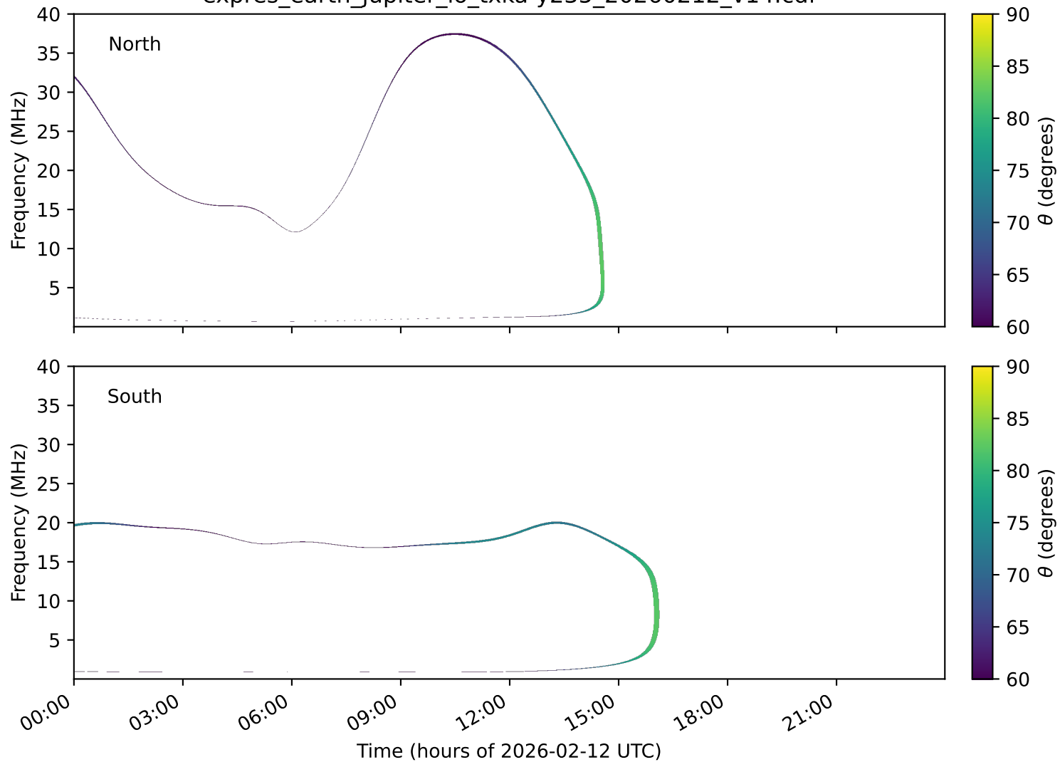
expres_earth_jupiter_io_txka-y235_20260212_v14.cdf
