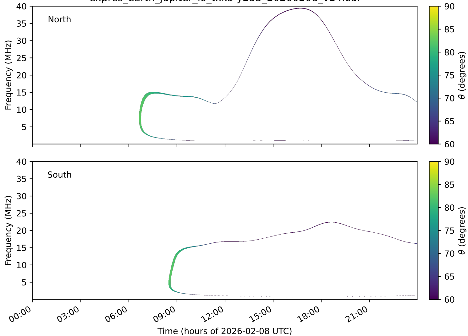
expres_earth_jupiter_io_txka-y235_20260208_v14.cdf
