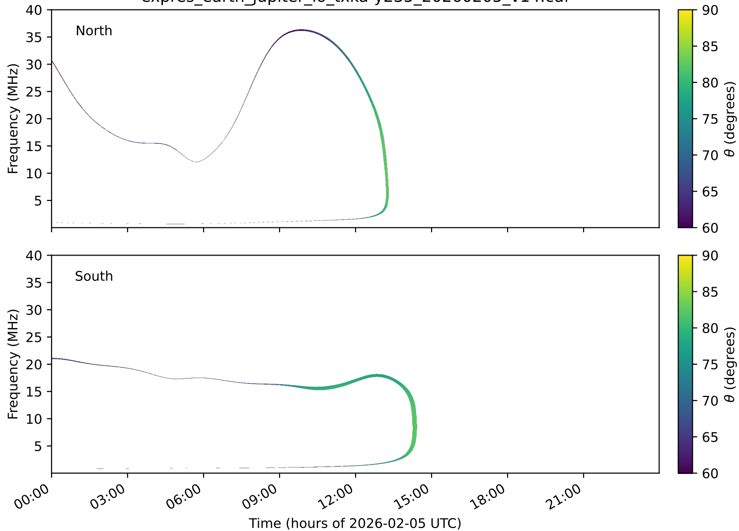
expres_earth_jupiter_io_txka-y235_20260205_v14.cdf
