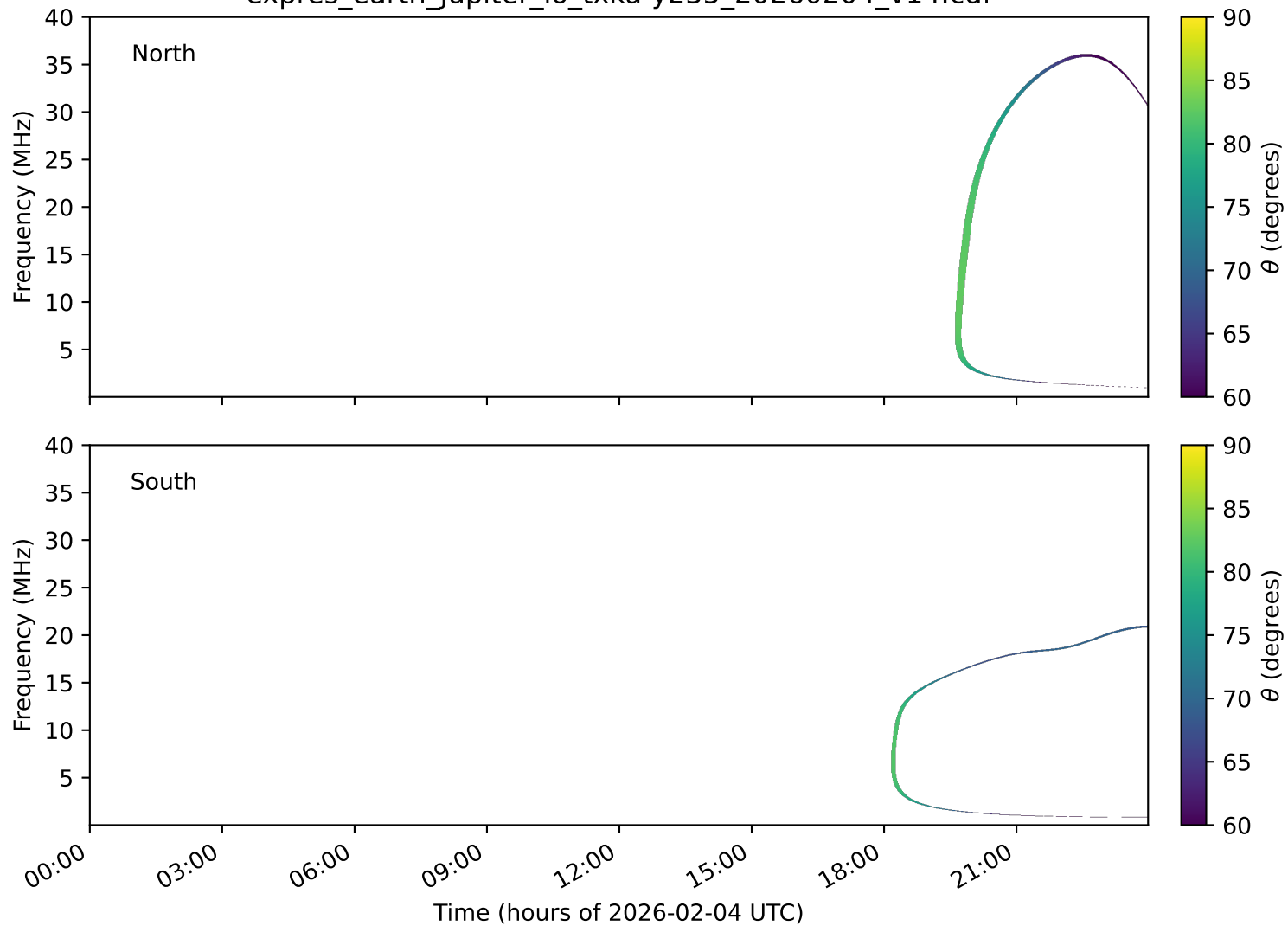
expres_earth_jupiter_io_txka-y235_20260204_v14.cdf
