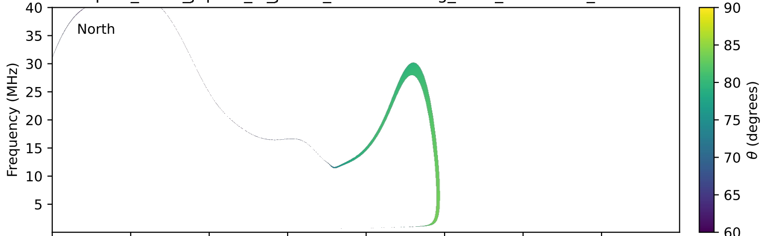
expres_earth_jupiter_io_jrm33_lossc-wid1deg_3kev_20260228_v11.cdf
